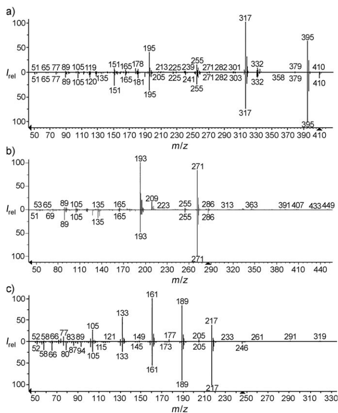
Figure 3. Mass spectra of a) \text{Ph}_2\text{MeSiOSiMe}_2\text{Ph} , b) \text{PhMe}_2\text{SiOSiMe}_2\text{Ph} , and c) \text{Et}_3\text{SiOSiEt}_3 formed in the reactions presented (top) and the literature spectra (bottom).
