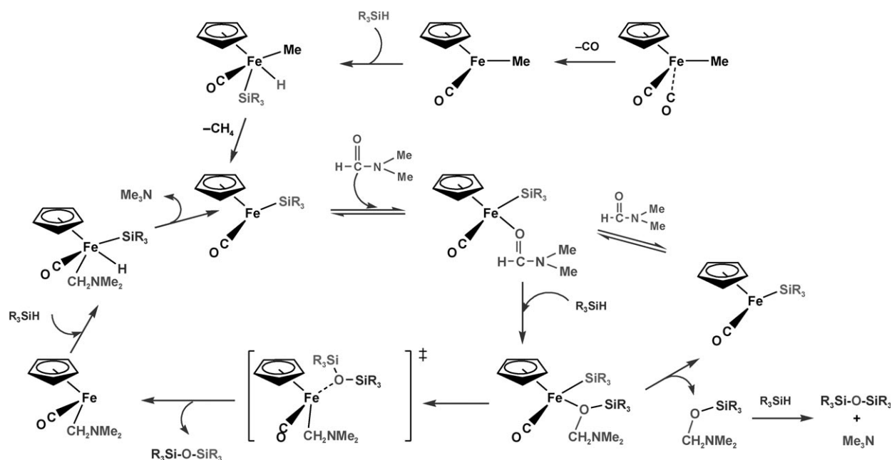
Scheme 1. Proposed catalytic mechanism for transformation of R_3SiH to R_3SiOSiR_3 .
